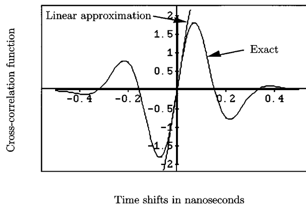
Fig. 3. Cross correlation \tilde{R}_w(\tau) between the received waveform of Fig. 1 and the pulse correlator waveform w_{\text{cor}}(t) (chosen equal to (d/dt)w_{\text{rec}}(t) of Fig. 1). In this example, the linear approximation (also shown) appears reasonable as long as \tau \leq 0.03 nanoseconds.
