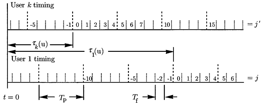
Fig. 7. Timing diagram, illustrating epochs and indexes for the signals received from user 1 and user k , with N_p = 5 (for this illustration only). The indexing begins from the zero reference time of the each users.
