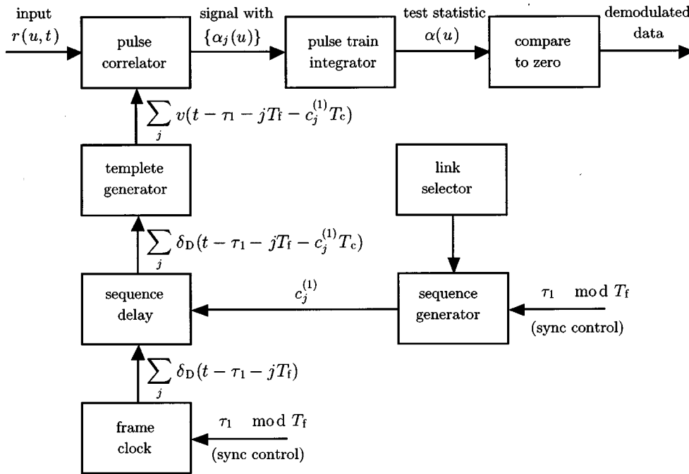
Fig. 4. Receiver block diagram for the reception of the first user's signal. Clock pulses are denoted by Dirac delta functions \delta_D(\cdot) .
